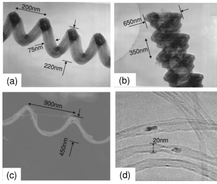
FIG. 2. Transmission electron microscope (TEM) micrographs of (a) singly wound, or (b) doubly wound, coiled carbon nanofibers (NF) synthesized through thermal CVD at high In concentration ( \text{In/Fe} ratio >3 ). (c) Scanning electron microscope (SEM) micrograph of nanotube (NT) bundles obtained at lower indium concentrations ( \text{In/Fe} ratio <2 ). (d) High resolution TEM (HRTEM) of the constituent tubes in (c) shows the random location of Fe-based catalyst particles throughout the NT.
